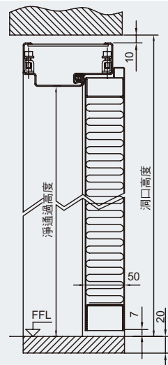
HAD 折邊門縱向視圖
