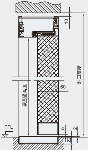
HC60SDC 縱向視圖
