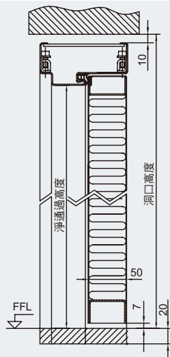
HAS 平口門縱向視圖
